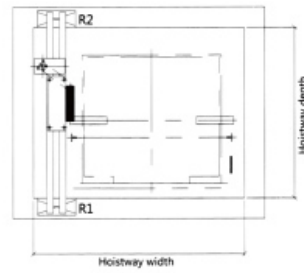
Overhead plan layout
