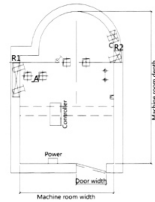
Machine room plan layout
